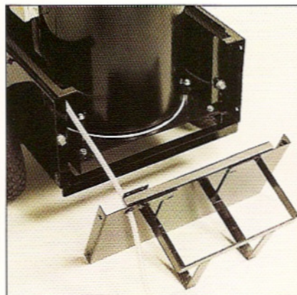
Removable Panel
